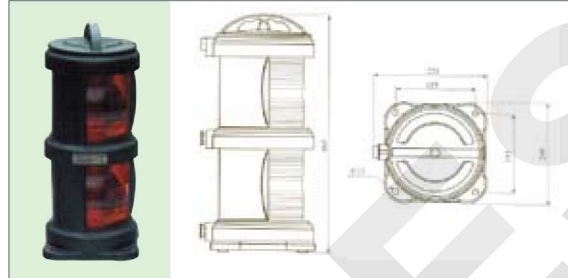
CXH2-101P - full plastic double - deck port light
