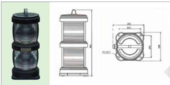
CXH3-101P - full plastic double - deck masthead light
